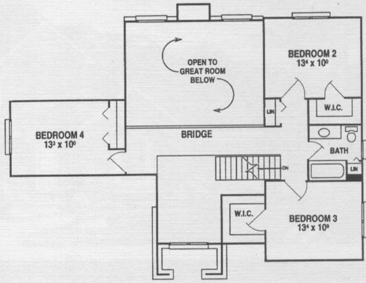
SECOND FLOOR • OPTIONAL 4 BEDROOM
